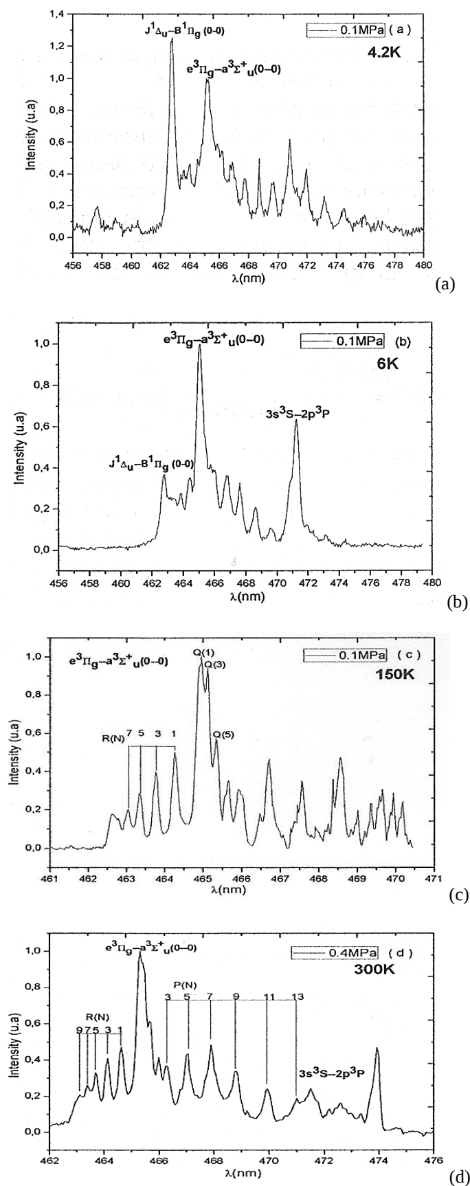
Fig. 2 – Bands of the triplet e^3\Pi_g-a^3\Sigma^+_u and singlet J^1\Delta_u-B^1\Pi_g transitions
