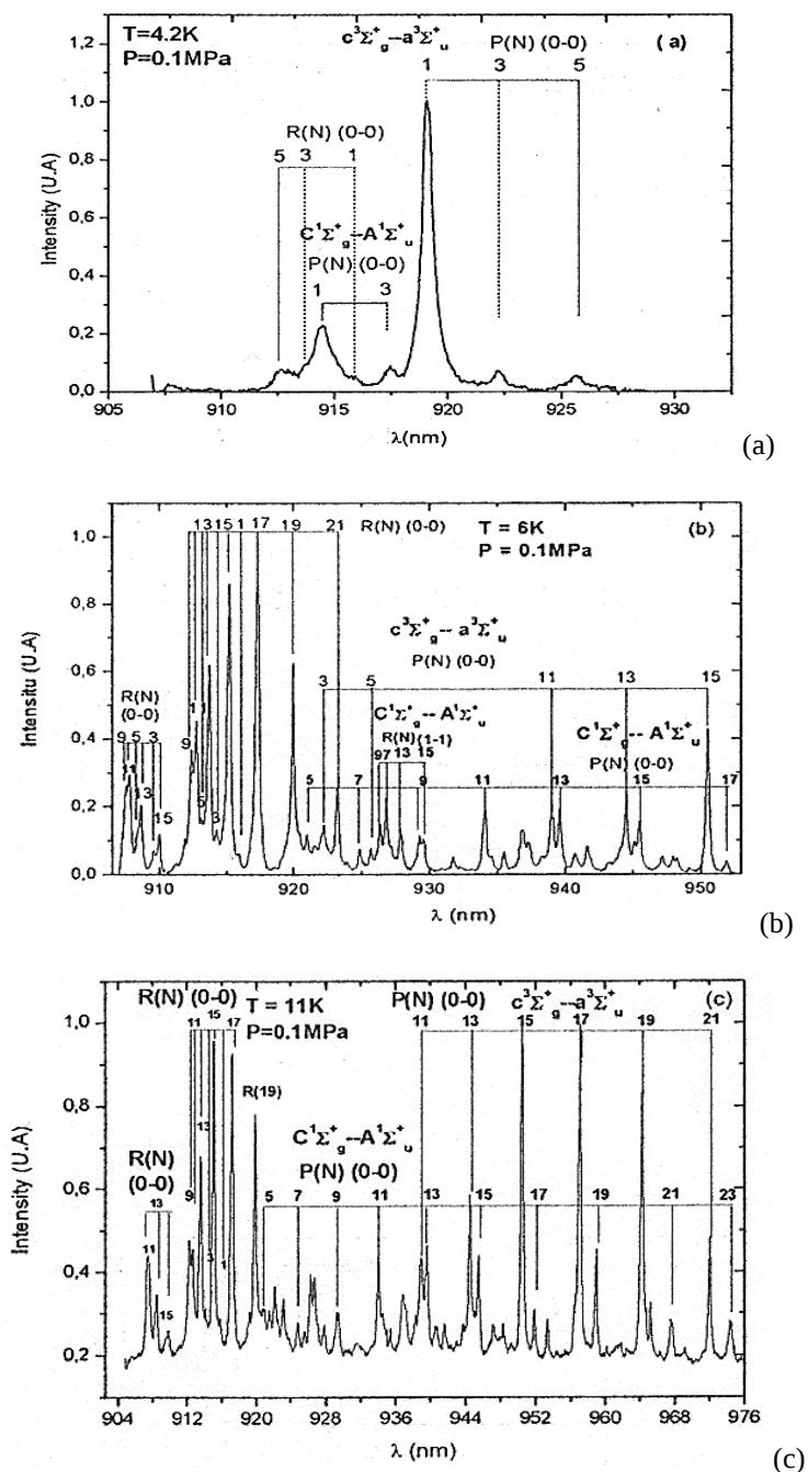
Fig 3 – Position of the rotational lines for (0-0) and (1-1) bands of the triplet c^3\Sigma_g^+ - a^3\Sigma_u^+ and singlet C^1\Sigma_g^+ - A^1\Sigma_u^+ transitions
