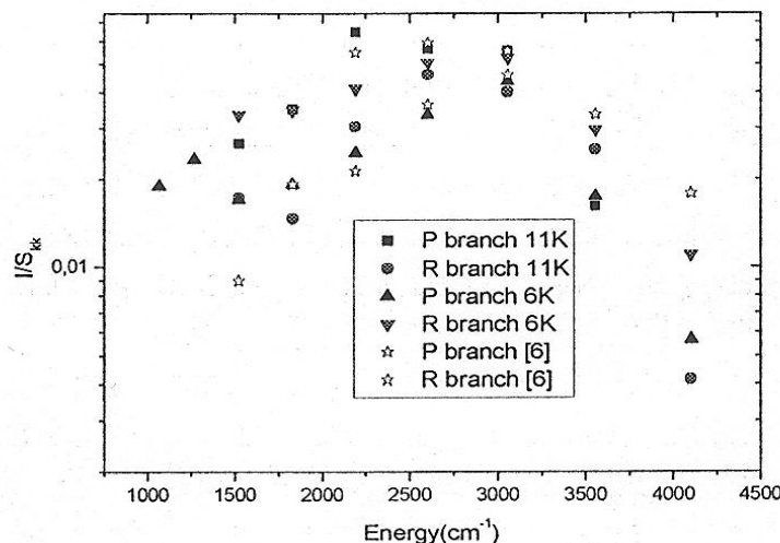
Fig. 5 – Values of \ln[I_{k'k''}/(v_{k'k''}^4 S_{k'k''})] against E_{k'} plot of the intensities in the P and R branches of the triplet c_3\Sigma^+_g - a^3\Sigma^+_u transition
