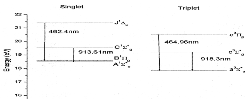
Fig 4 – The energy level diagram of molecular helium
